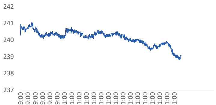
Figure 2 HNX-Index Intraday
