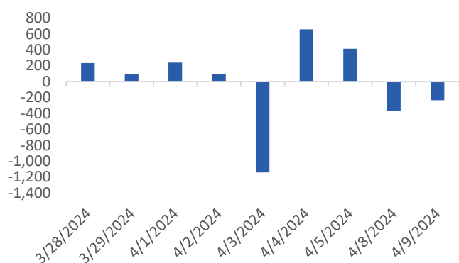
Figure 3 Proprietary trading
