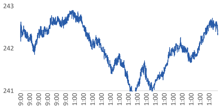
Figure 2 HNX-Index Intraday
